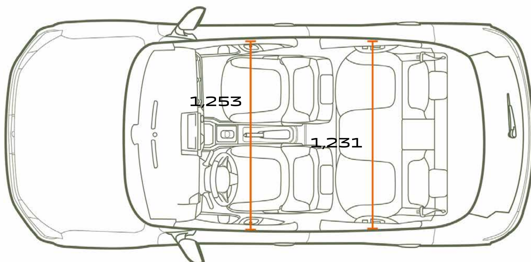
TOP VIEW
