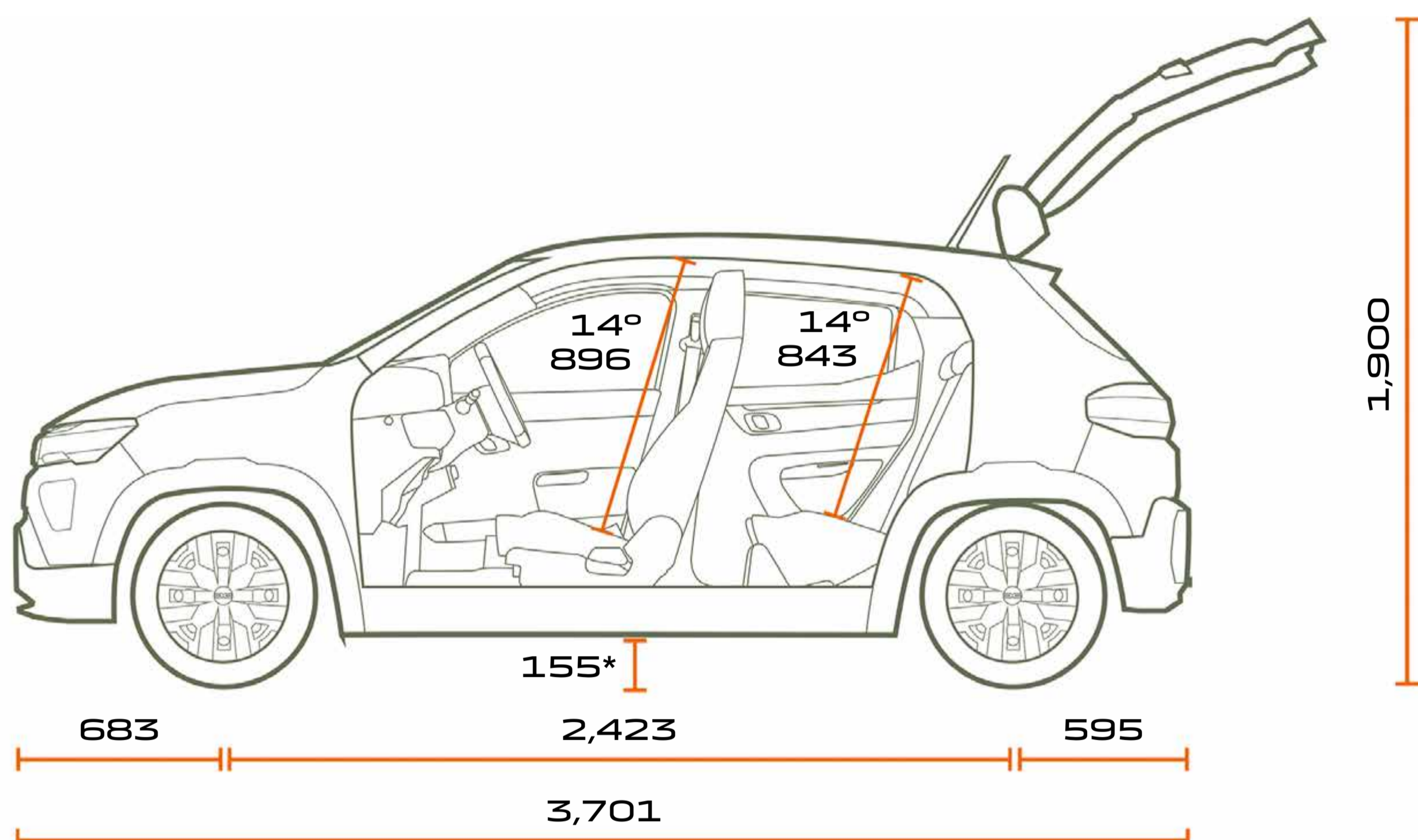
SIDE-FACE VIEW
